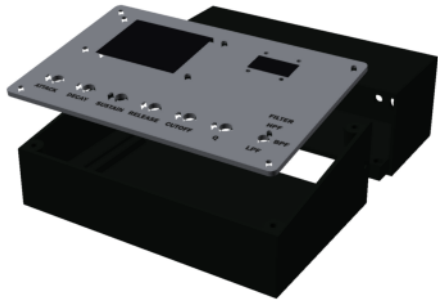
(b) despiece
